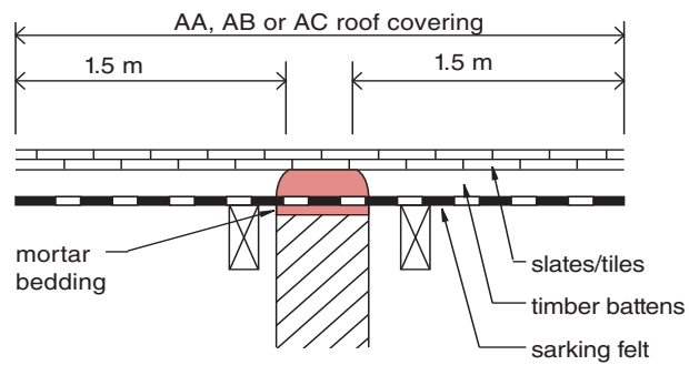
(b) Building of Purpose Group 1, 2(b), 3 or 5 not more than 15 m in height
