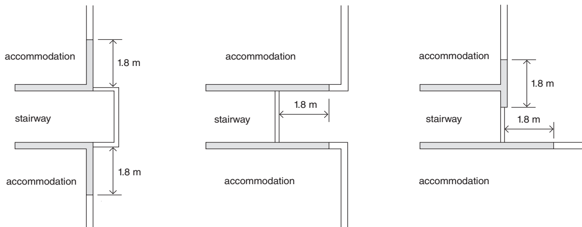
(a) projecting stairway
