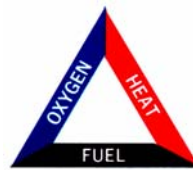
Figure 2: Fire Triangle
