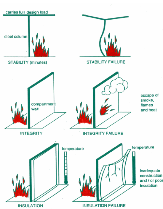
Figure 3: Fire Resistance performance criteria
